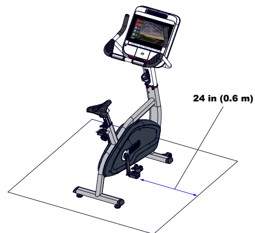
Fig. 1 Required Clearance
